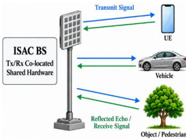
Figure 5.1 Architecture of a Monostatic ISAC System
