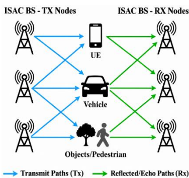
Figure 5.3 Architecture of a Multistatic ISAC System.
