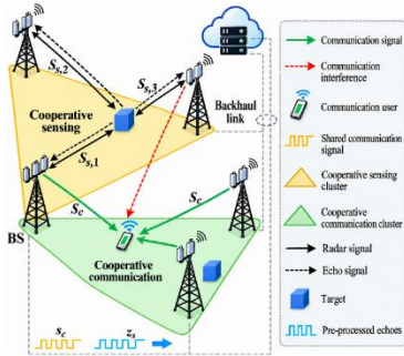
Figure 5.9 Architecture of cooperative ISAC System.
