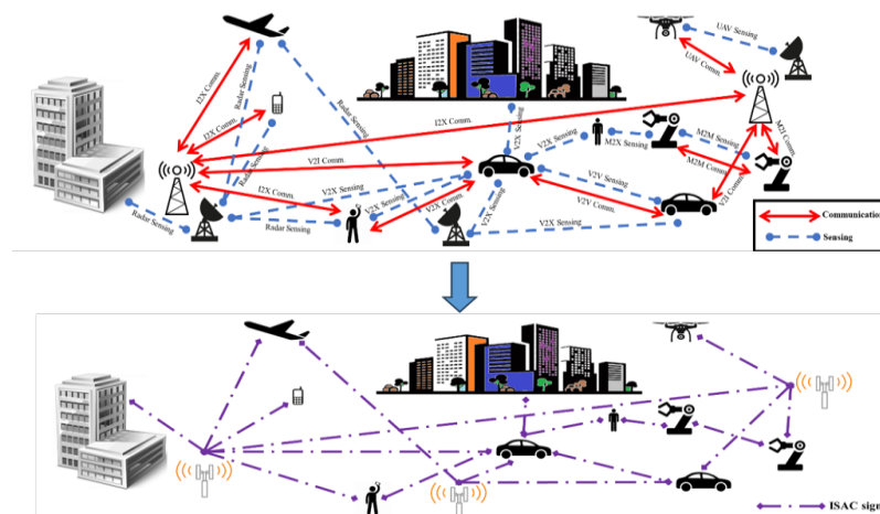
Fig. 2.1. Comparison of traditional scenarios, where communication and radar have separate infrastructure requirements (above part), with ISAC-enabled joint sensing and communication
