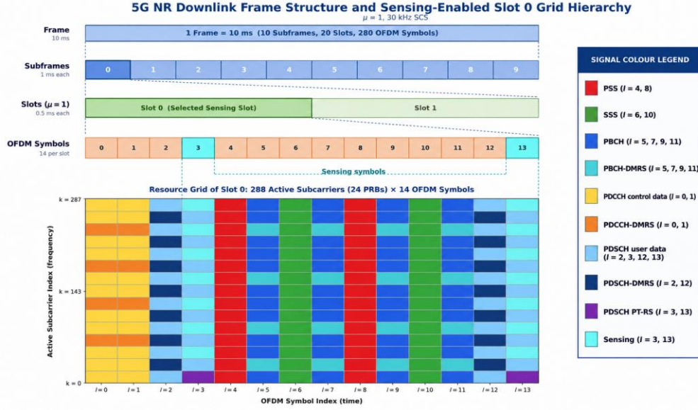
Fig. 3.2. NR-inspired experimental ISAC frame structure.
