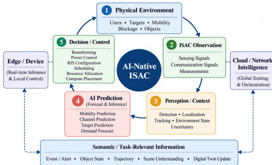
Fig. 8.1. Closed perception–decision loop in AI-native ISAC, integrating environmental sensing, context extraction, AI-driven prediction, network control, and edge–cloud intelligence.
