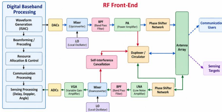
Fig. 4.2 Block diagram of FD ISAC transceiver and SIC cancellation.
