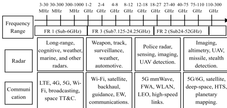
Figure 1.3. Frequency-spectrum coexistence of radar sensing and wireless communication systems.
