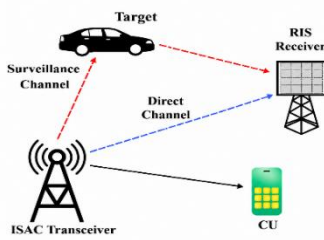
Fig. 5.5 Passive ISAC System.
