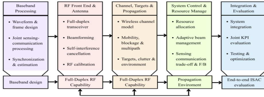
Figure 4.1: End-to-end ISAC system architecture highlighting RF and FD antenna technologies
