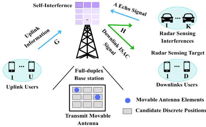
Figure 4.3. Multi-stage SIC in an FD ISAC transceiver.
