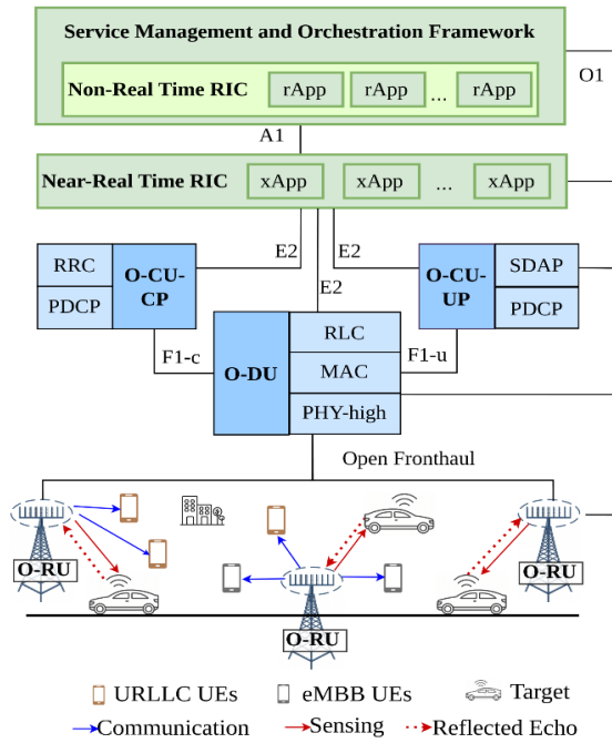
Figure 6.1 Architecture of the O-RAN-based ISAC Network.
