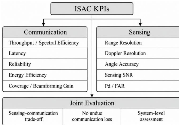
Fig. 2.3. Hierarchical categorization of KPIs for ISAC evaluation.
