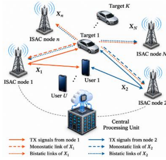
Figure 5.8 Architecture of Distributed ISAC System.
