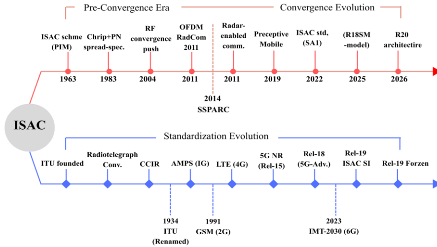
Fig. 1.2 Parallel evolution of ISAC technologies and mobile communication standards.
