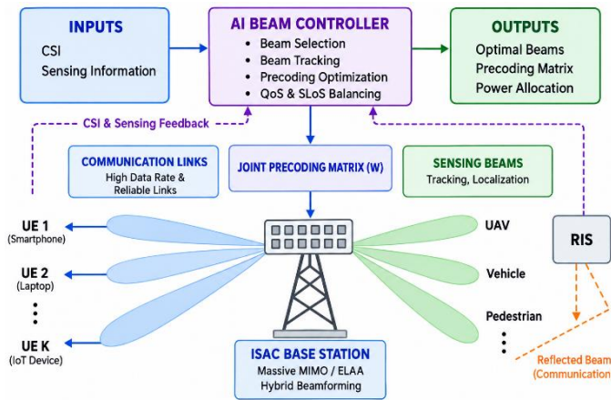
Fig 4.4. AI-assisted joint beamforming and precoding architecture for native 6G ISAC.
