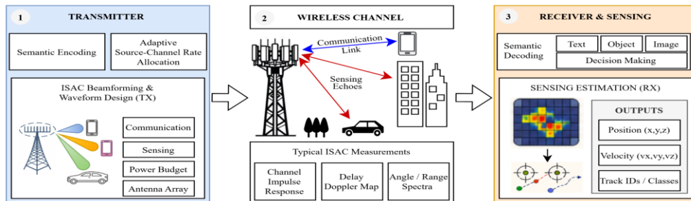
Fig. 6.3. AI-native RAN architecture for integrated communication and sensing with real-time AI processing.
