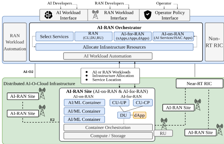
Figure 6.2 Architecture of the AI-native ISAC Network.
