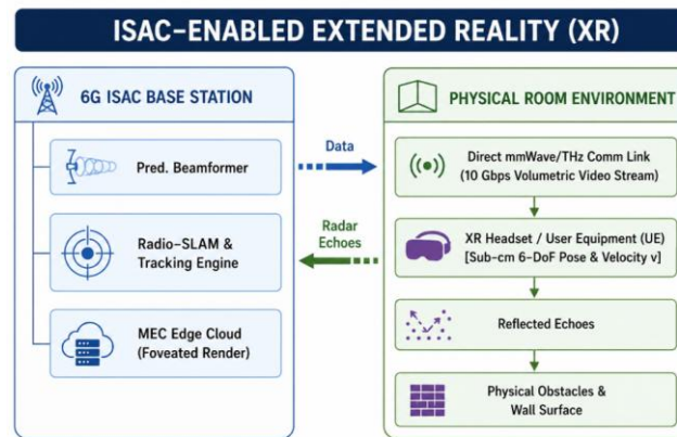
Figure 13.3: Conceptual architecture of an ISAC-enabled 6G wireless network supporting immersive XR [7]
