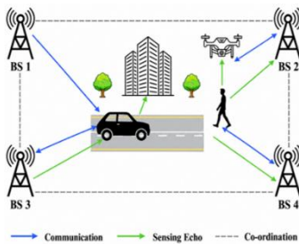
Fig. 5.6 Infrastructure-based ISAC.
