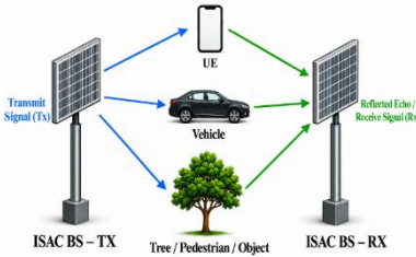
Figure 5.2 Architecture of a Bistatic ISAC System.
