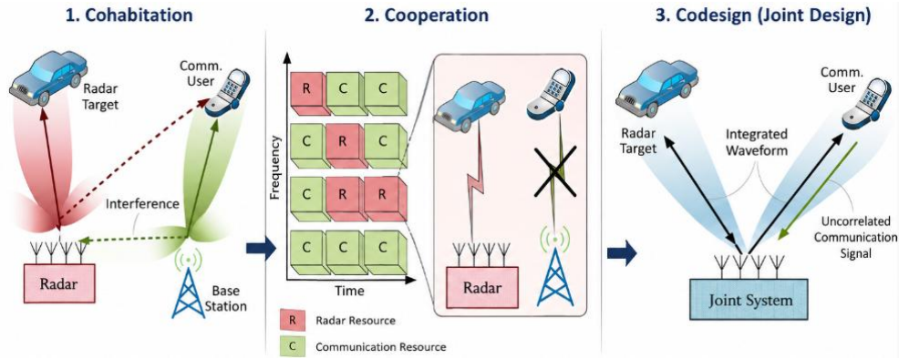
Fig. 3.3 Evolution paradigms of radar-communication integration: (1) Cohabitation, (2) Cooperation, and (3) Codesign, with an ISAC framework and unified hardware and integrated waveforms.
