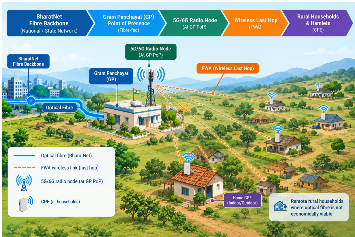
Figure 6.2. The gram-panchayat-anchored model: a BharatNet fibre point of presence at the gram panchayat with an FWA last hop to surrounding households and hamlets.
