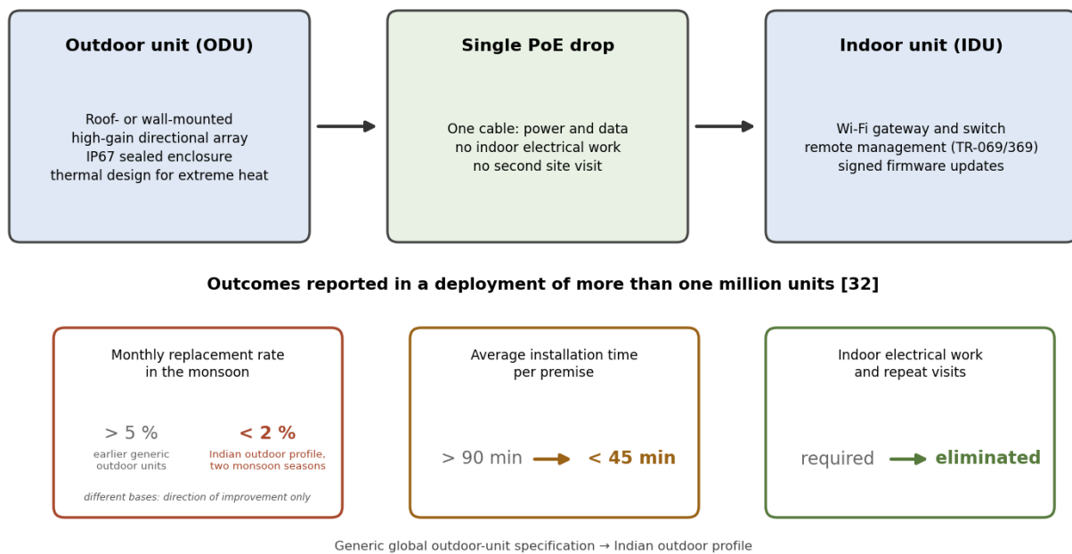
Figure 3.1. The Indian outdoor profile: split-architecture CPE with a single PoE drop, and outcomes reported across two monsoon seasons in a deployment of more than one million units [32].
