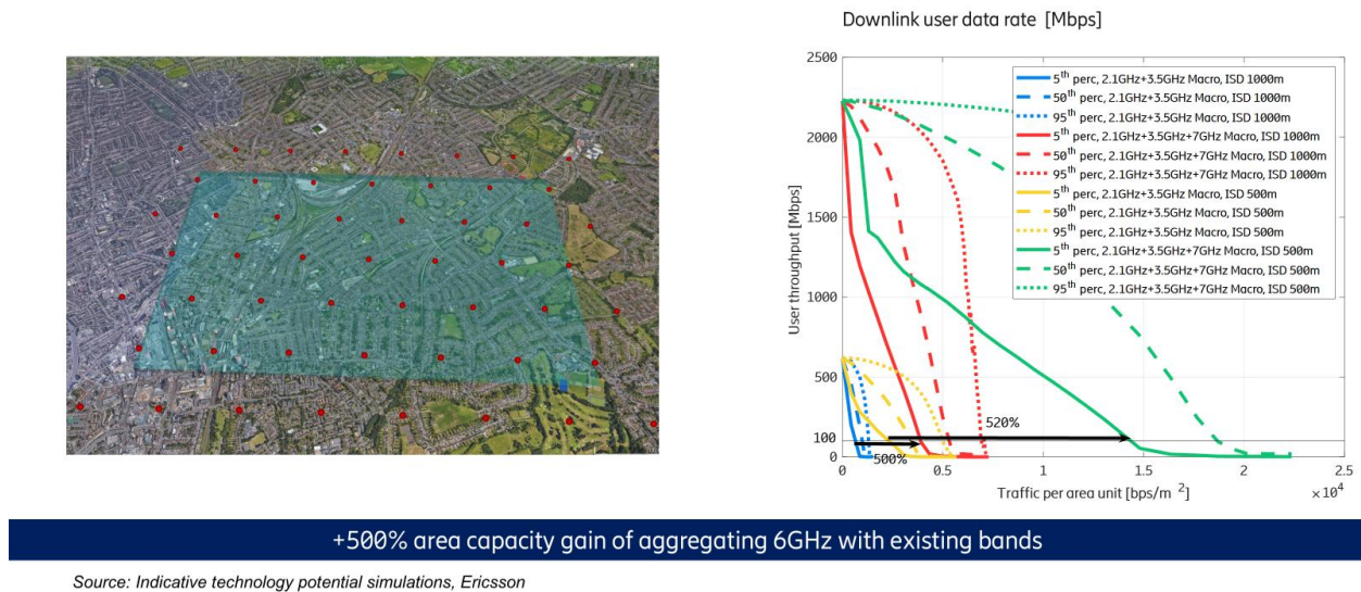
Figure 7.2. Area capacity when 200 MHz of 6-8 GHz TDD spectrum is aggregated with existing bands (vendor simulation, UK suburban layout, downlink only). Baseline deployment: 2.1 GHz and 3.5 GHz; inter-site distance 500 m and 1000 m.
