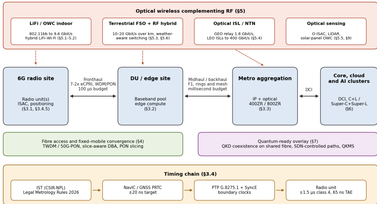
Figure 2.1. The converged RF–optical 6G infrastructure covered in this paper, with the section that treats each element.
