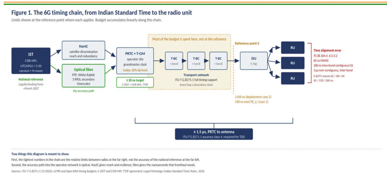
Figure 3.2. The 6G timing chain from Indian Standard Time to the radio unit.
