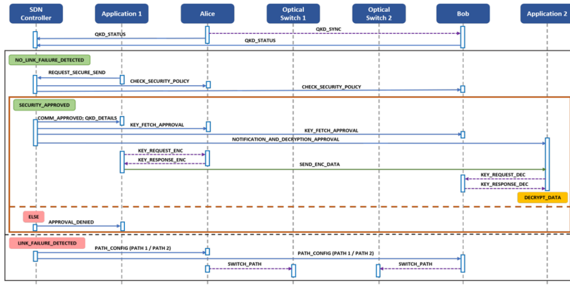
Figure 7.3. System interaction sequence for SDN-enabled QKD path provisioning
