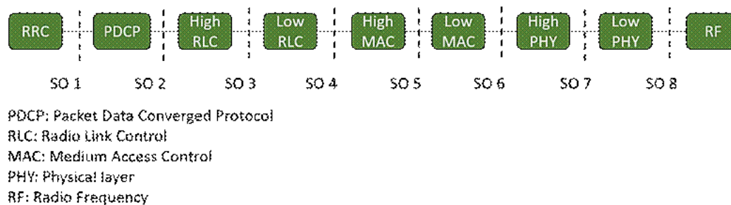
Figure 3.1. Split options in the RAN architecture [14].
