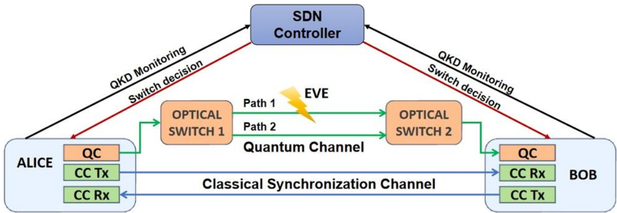
Figure 7.2. SDN-based threat detection and adaptive recovery.
