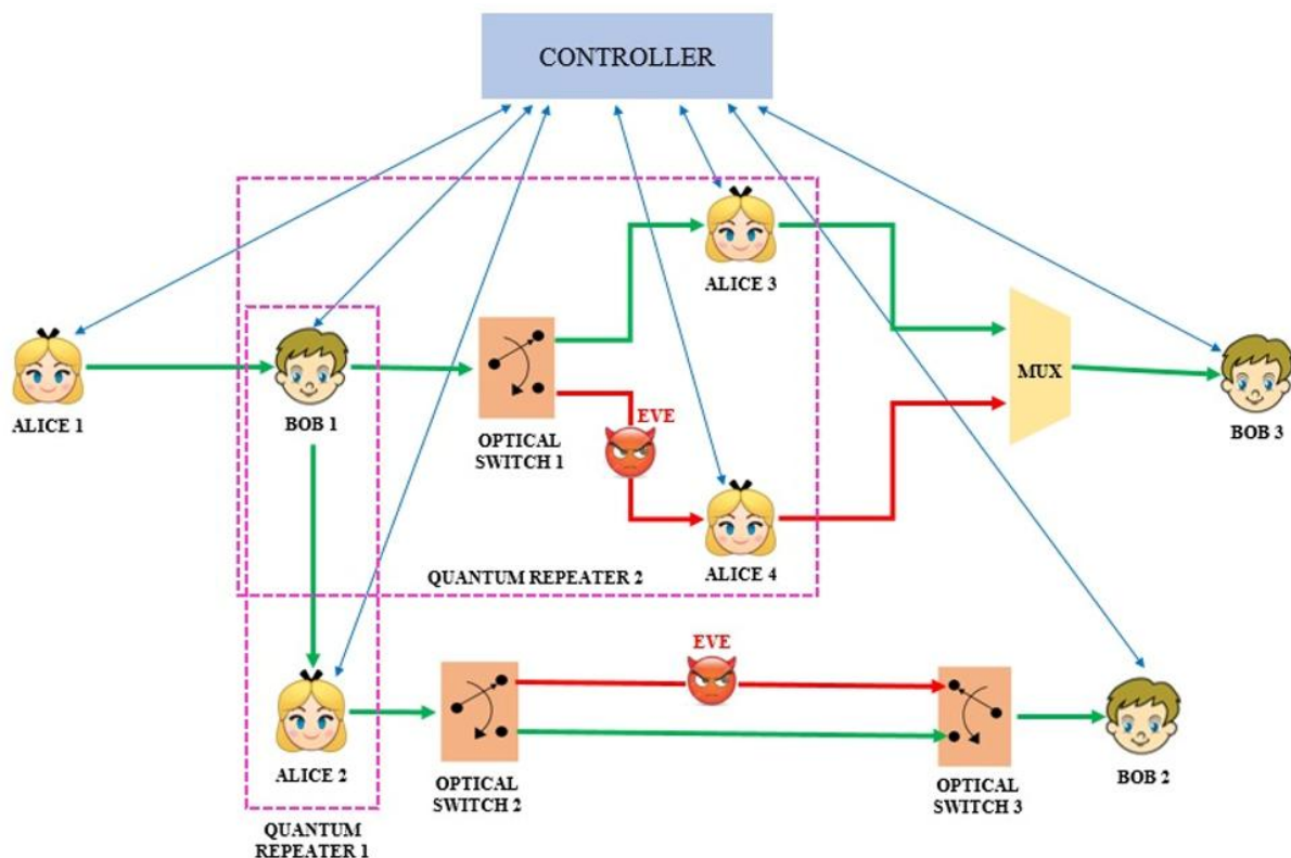
Figure 7.1. SDN-based optical network for QKD.
