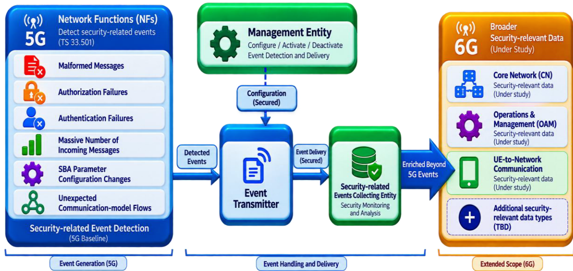
Figure 6: Security related events collection
