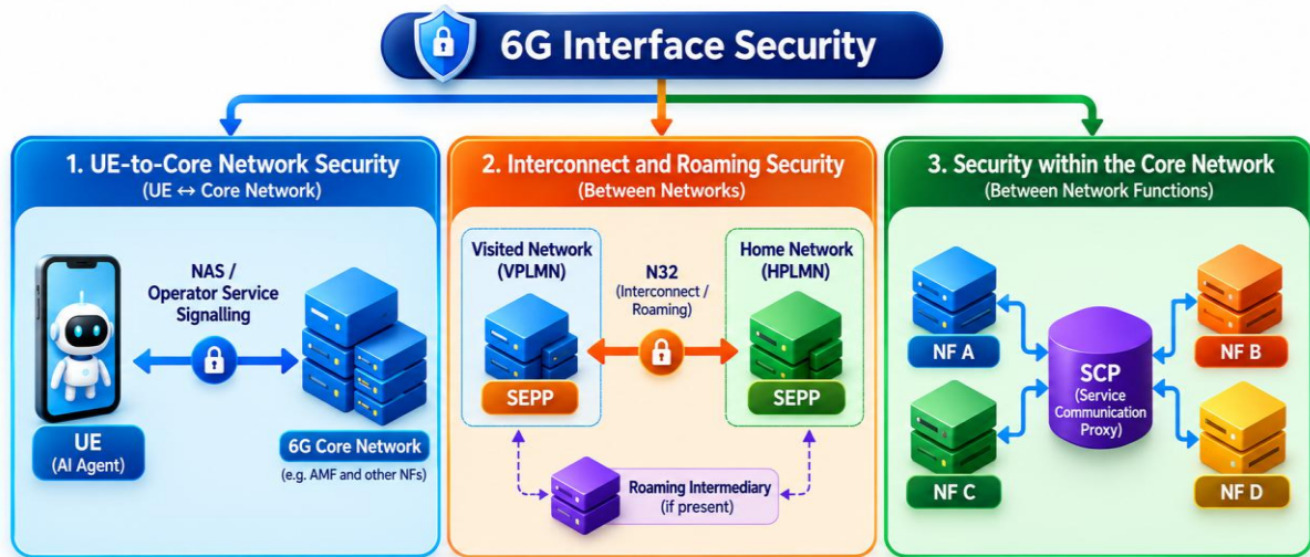
Figure 5: Interface Security
