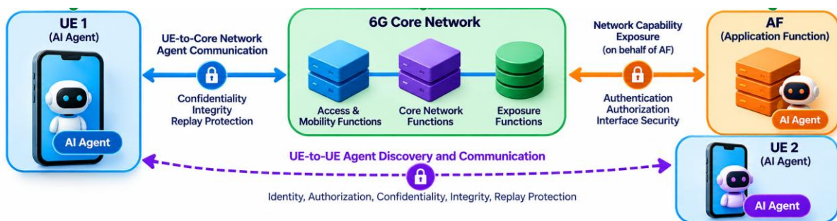
Figure 7: AI Security
