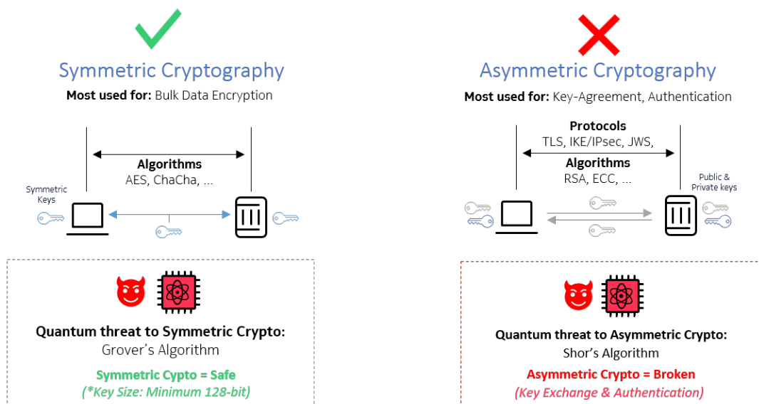
Figure 2: Quantum Threats to Symmetric and Asymmetric Cryptography
